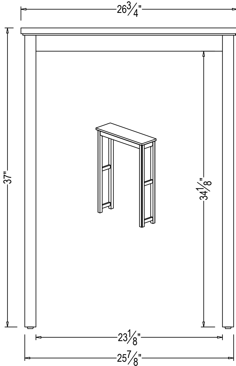
ANVA72WH DORSET TOILET BASE
